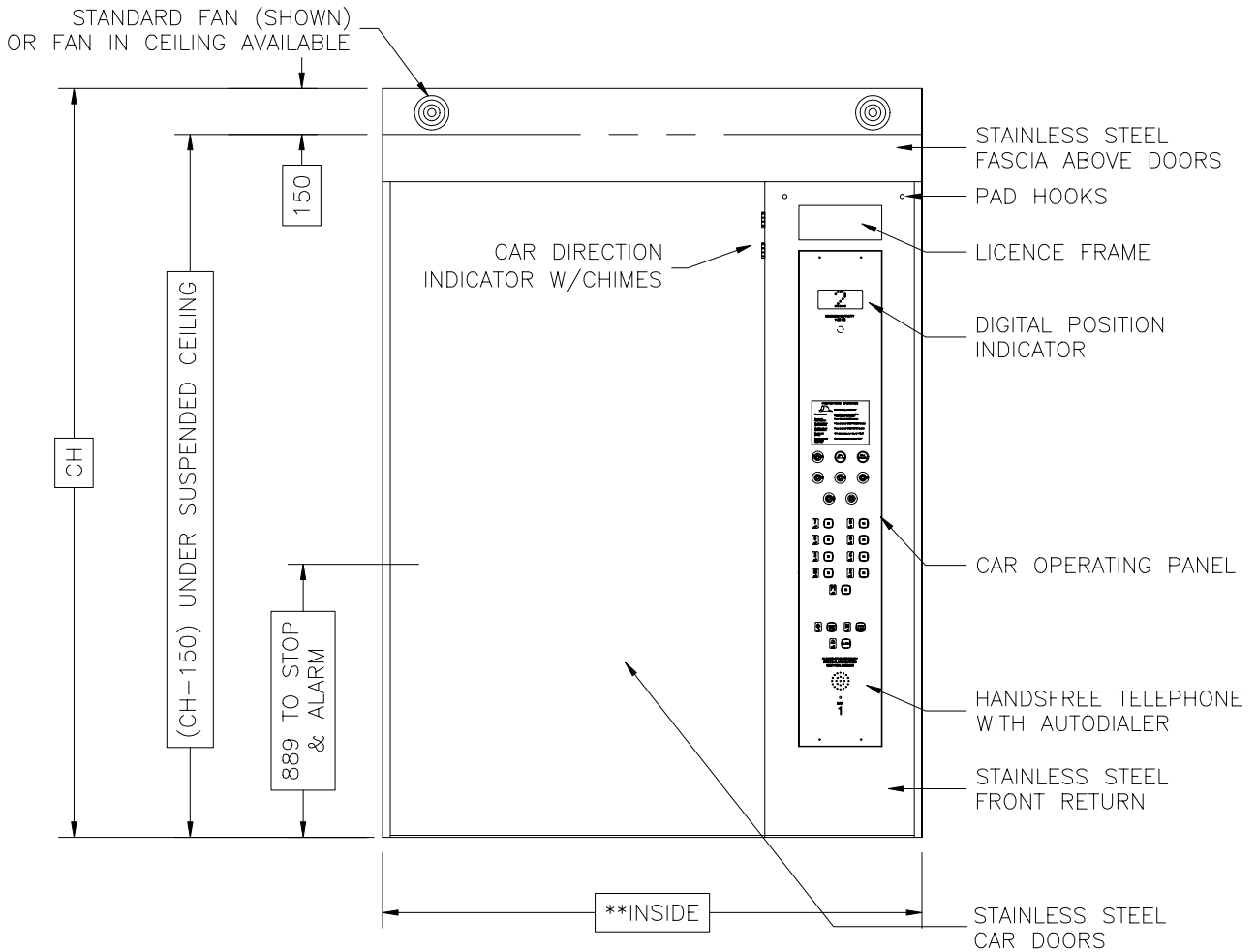
SIDE OPENING DOORS
