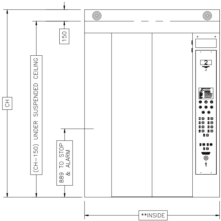
CENTRE OPENING DOORS
