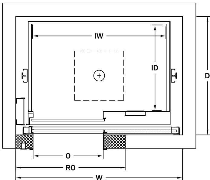
Left Hand Opening Shown Right Hand Opposite
